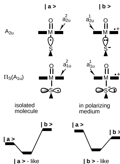
Figure 4. Resonance structures ( |a> and |b> ), which contribute to the "redox mesomerism" in the A_{2u} and \Pi_S states of 1 ; L=HS, and their mixing in the isolated molecule and in a polarizing medium.
